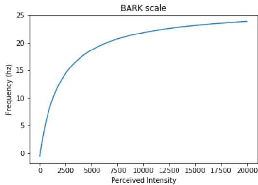
Figure 4: The BARK scale is a psychoacoustic model of the human perception of loudness in relation to frequency. The scale suggests that humans perceive high frequencies as louder than lower frequencies. The perceived intensity values associated with each frequency correspond to the first 24 critical bands of hearing.
