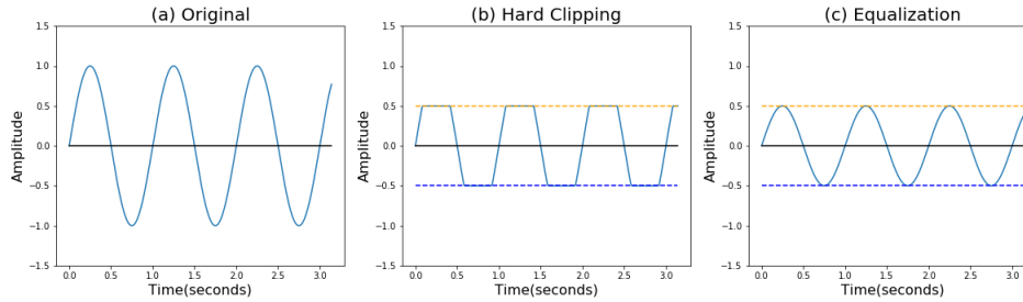
Figure 2: The figure above demonstrates the effects on an of (b) Hard Clipping and (c) Equalization on an (a) Original signal. We can see that (b) Hard Clipping results in a distortion of the audio signal, making the audio noisier. In contrast, (c) Equalization reduces the intensity of a single frequency in the signal, avoiding any audible distortion. It is important to note that equalization does not just reduce the intensity of the whole signal, but only a particular frequency of the signal.
