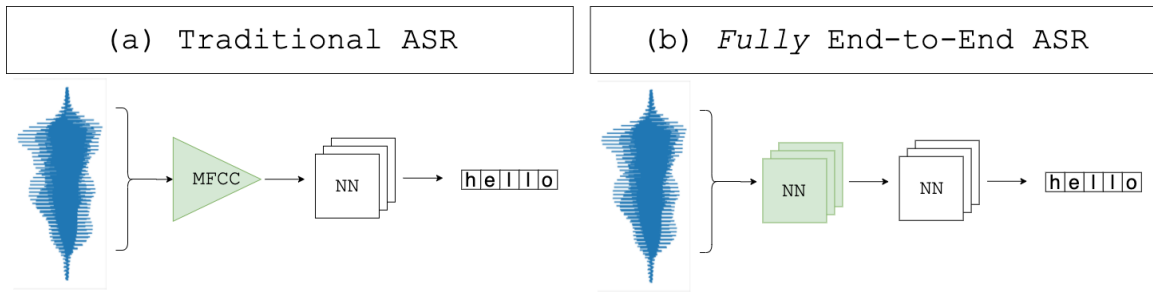
Figure 1: The architectures of (a) traditional and (b) fully end-to-end ASRs. The primary difference between the two is that fully end-to-end ASRs do not include any signal processing-based feature extraction algorithms (e.g., MFCC). Instead, they use NNs that learn to extract the appropriate features during model training.
